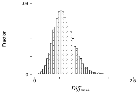
Figure 2.4.2 10,000 Diff_{max4} values generated under proportional hazards
