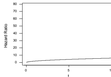
Figure 3.2.1 Increasing hazards.
