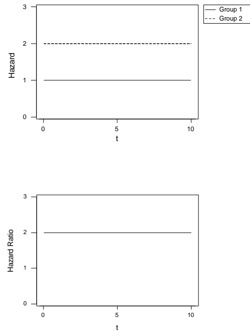
Figure 3.1.1 Constant hazards.
