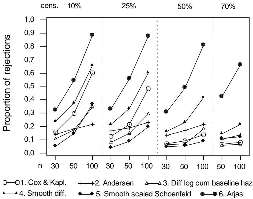
Figure 3.4.2 Crossing hazards
