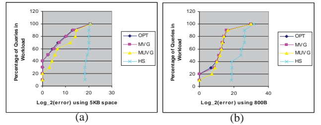
Figure 2: Performances on (a) SwetoDBLP and (b) LUBM2
