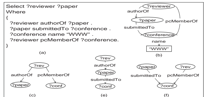
Figure 1: A graph pattern query and its sub-graph patterns.
