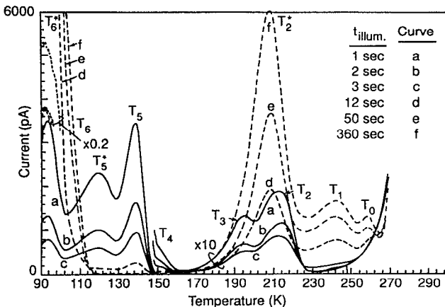
FIG. 2. TSC spectra under different illumination times from 1 to 360 s, showing a drastic change in the TSC spectrum from feature I to II at t_{\text{illum}} \sim 12 s (maximum light intensity used).
