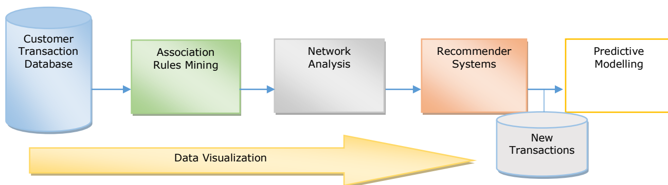
Figure 2: Exercise's Workflow
