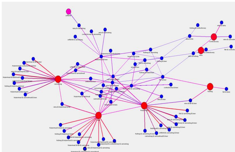
Figure 6: Link Graph
