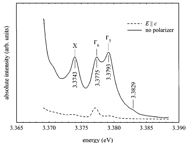
FIG. 3. Unpolarized and \mathbf{E} \parallel \mathbf{c} -polarized free-exciton-like transitions.
