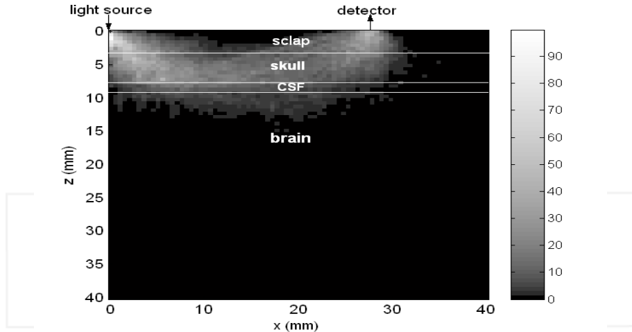
Fig. 9. Spatial sensitivity profile of photons in 2D three-layer head model as given by MC simulation for a single source- detector separation. Light in the near-infrared range (700-900 nm), compared to the visible light range penetrates tissues more deeply. The photons change direction multiples times as they scatter, and they follow a generally curved path called the “banana shaped” curve between the light source and the detector location at the surface (Mansouri and L’Huillier, 2007).
