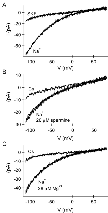
FIGURE 10. Pharmacological properties of monovalent CRAC current. CRAC current was allowed to develop in external \text{Ca}^{2+} and \text{Na}^+ current through CRAC channels was recorded in \text{Na}^+ -HEDTA. The internal solution contained: 12 EGTA, and 6 (3 mM free) \text{Mg}^{2+} . (A) Effect of 20 \mu\text{M} SKF-96365 on \text{Na}^+ current through CRAC channels. SKF block was fully reversible. (B) I-V of \text{Na}^+ current through CRAC channels in the presence and absence of 20 \mu\text{M} spermine. (C) I-V of \text{Na}^+ current through CRAC channels in the presence and absence of 28 \mu\text{M} external \text{Mg}^{2+} , a free \text{Mg}^{2+} concentration that effectively blocks MIC current (Fig. 4 B). At the end of the experiment (B and C) external \text{Na}^+ -HEDTA was substituted by \text{Cs}^+ -HEDTA; the loss of inward current confirms that the monovalent current is through CRAC channels.
