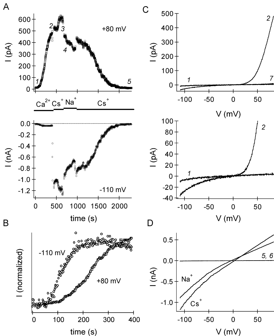
FIGURE 1. Development and run-down of CRAC and MIC currents in the presence and absence of external divalent ions. Internal solution contained 12 mM EGTA and no added \text{Mg}^{2+} . (A) Outward (top) and inward (bottom) current development in 2 mM external \text{Ca}^{2+} , followed at \sim 400 s by exposure to \text{Cs}^+ —then \text{Na}^+ -HEDTA. MIC ran down gradually over 2,000 s. (B) Current development time course for inward and outward currents compared. The scaled and inverted inward current measured at -110 mV is shown superimposed with the outward current (80 mV). The inward current clearly precedes the development of the outward current, despite its smaller size. (C) I-V plots of MIC current in 2 mM \text{Ca}^{2+} plotted with two different current amplitude scales. Traces 1 and 2 correspond to times indicated in A. Trace 7 was collected 51 min after break-in after reintroduction of 2 mM \text{Ca}^{2+} . (D) I-V plots of monovalent MIC current in \text{Na}^+ - and \text{Cs}^+ -HEDTA. Both \text{Cs}^+ and \text{Na}^+ are permeant through the channel. The indistinguishable traces 5 and 6 (taken 54 min after break-in) were obtained in \text{Cs}^+ and \text{Na}^+ solution, respectively, after complete run-down of MIC current.
