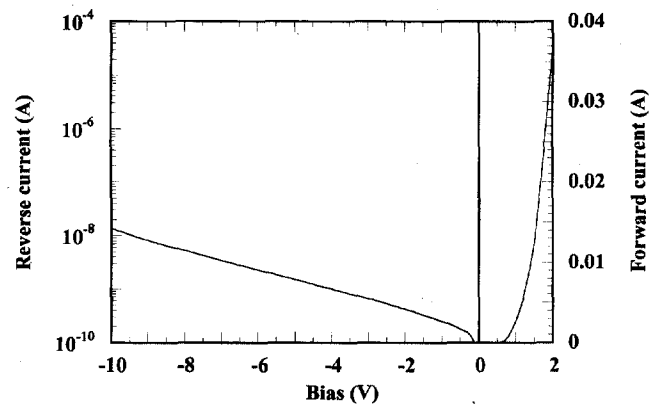
FIG. 6. Typical I – V curve for the Schottky diodes fabricated from the Si-doped layer grown with 60 sccm ammonia flow rate.
