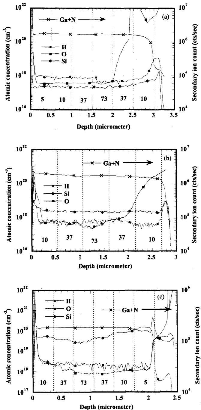
FIG. 1. Depth profile of Si, H, and O for three Si-doped films grown on highly resistive GaN/AlN buffer with three different Si levels. (a) \sim 2 \times 10^{17} \text{ cm}^{-3} , (b) \sim 3 \times 10^{18} \text{ cm}^{-3} , (c) \sim 5 \times 10^{19} \text{ cm}^{-3} . Shown together is the secondary ion count for matrix elements to mark the position of interface between substrate and film. The numbers in each segment are the ammonia flow rate used for that segment.
