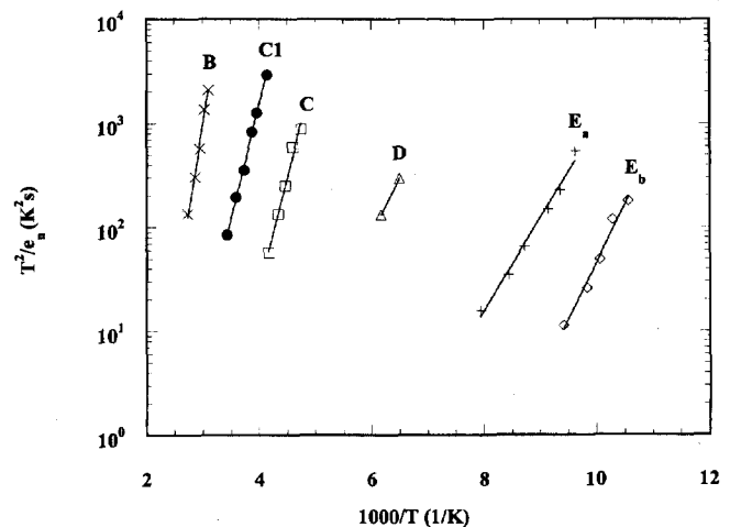
FIG. 7. Arrhenius plots of T^2/e_n vs 1000/T for deep levels observed in MOCVD, HVPE, and RMBE-grown GaN Schottky diodes, where e_n is electron emission ratio. The trap signatures for deep levels B, C, D, E_a , and E_b were obtained from MOCVD and HVPE samples (see Ref. 17) and C1 from RMBE samples.
