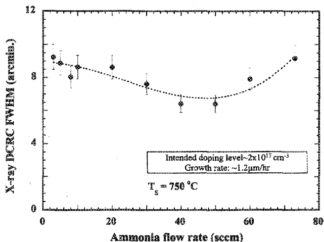
FIG. 3. Variation in FWHM of x-ray rocking curve for (0002) GaN plane of the Si-doped films grown with various ammonia flow rates on highly resistive GaN/AlN buffer.
