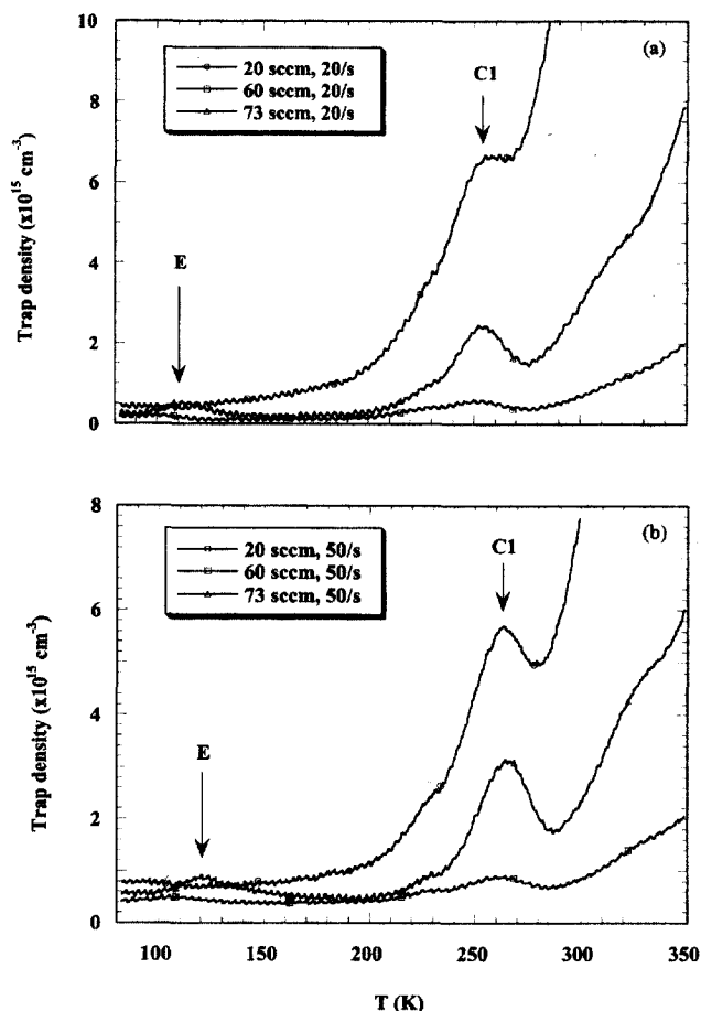
FIG. 8. DLTS spectra measured with rate windows of (a) 20/s and (b) 50/s for the three GaN Schottky diodes grown with three different ammonia flow rates.
