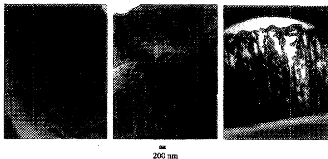
FIG. 5. XTEM images of Si-doped GaN films in set I. The ammonia flow rate used for the growth of Si-doped layer was (a) 5 sccm, (b) 50 sccm, (c) 73 sccm, respectively. The zone axis was slightly off from [11\bar{2}0] . The arrow in (b) indicates the approximate position of the interface between undoped GaN and Si-doped GaN.
