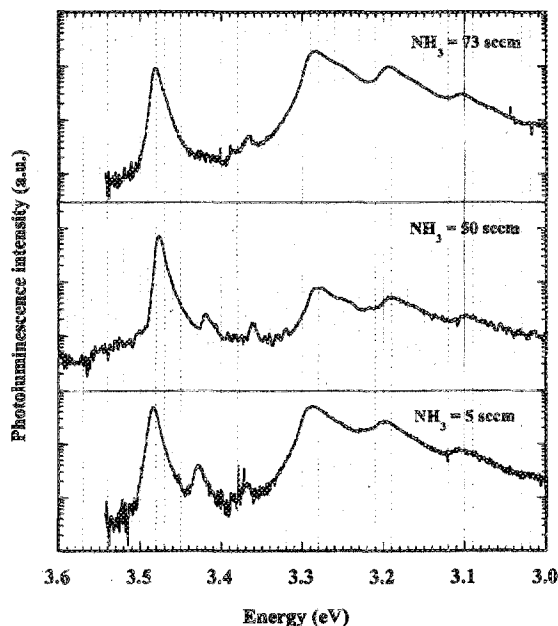
FIG. 4. Low-temperature (4.2 K) PL spectra of three Si-doped GaN films grown with different ammonia flow rates.
