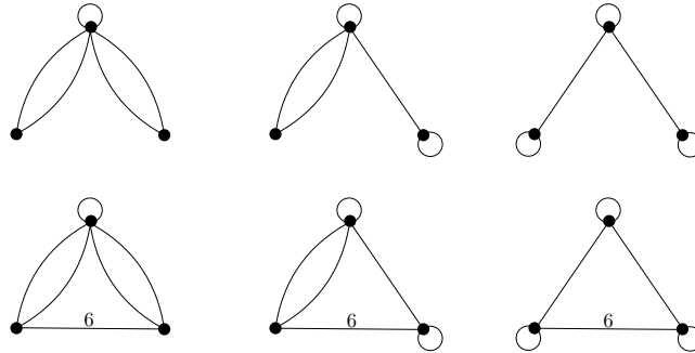
Figure 9: The sixth graph shown is the only bicircular representation of \mathcal{W}^3 .
