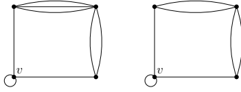
Figure 16: Graphs for the proof of Case 2.2.1.2.
