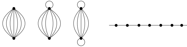
Figure 3: The matroid U_{2,7} and its bicircular representations.
