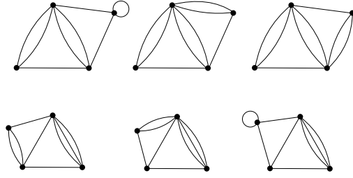
Figure 12: Graphs for the proof of Case 2.2.1.1.3
