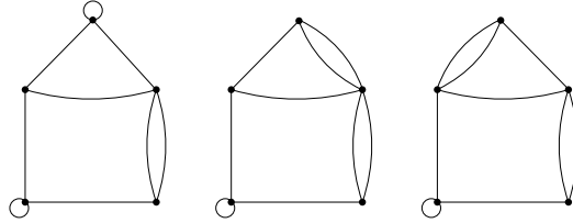
Figure 17: Graphs for the proof of Case 2.2.1.2
