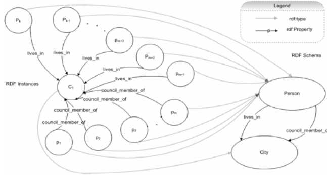
Fig. 1. Illustrative example for Instance Participation Distribution
