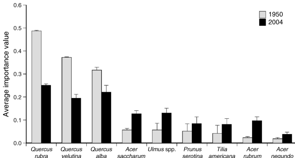
FIG. 2. Changes in the relative abundance of major canopy species. Species are ranked in decreasing abundance based on the original sample data (see Methods ). Error bars represent + 1 SE.
