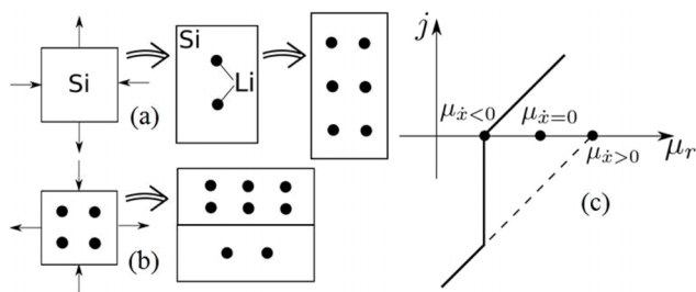
Figure 1 | (a) Anisotropic compositional deformation of Li_xSi during lithiation under deviatoric stresses. (b) When deviatoric stress S , applied to a sample, produces the same driving force for insertion and extraction, Li_xSi sample may be fluctuationaly divided into two samples separated by an interface, in one of which insertion occurs and in another one extraction takes place. (c) Magnitude of Li flux versus chemical potential of Li reservoir \mu_r under deviatoric stresses (solid line, Eq.(6)).
